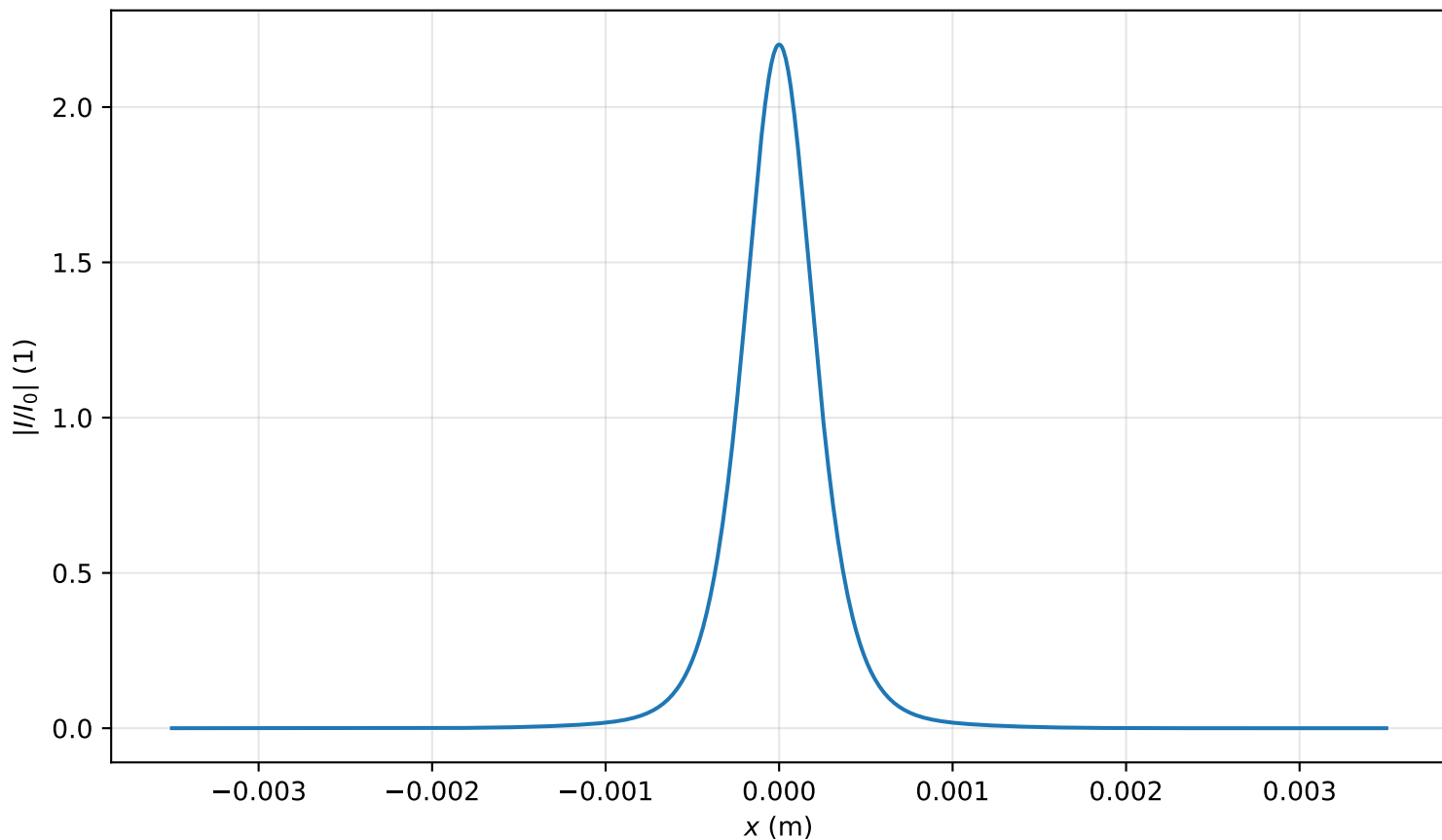
Intensity profile I(x, y = 0, z = 2.149m)/I_0 , P_{in}=1.0P_{cr} , artificial time
